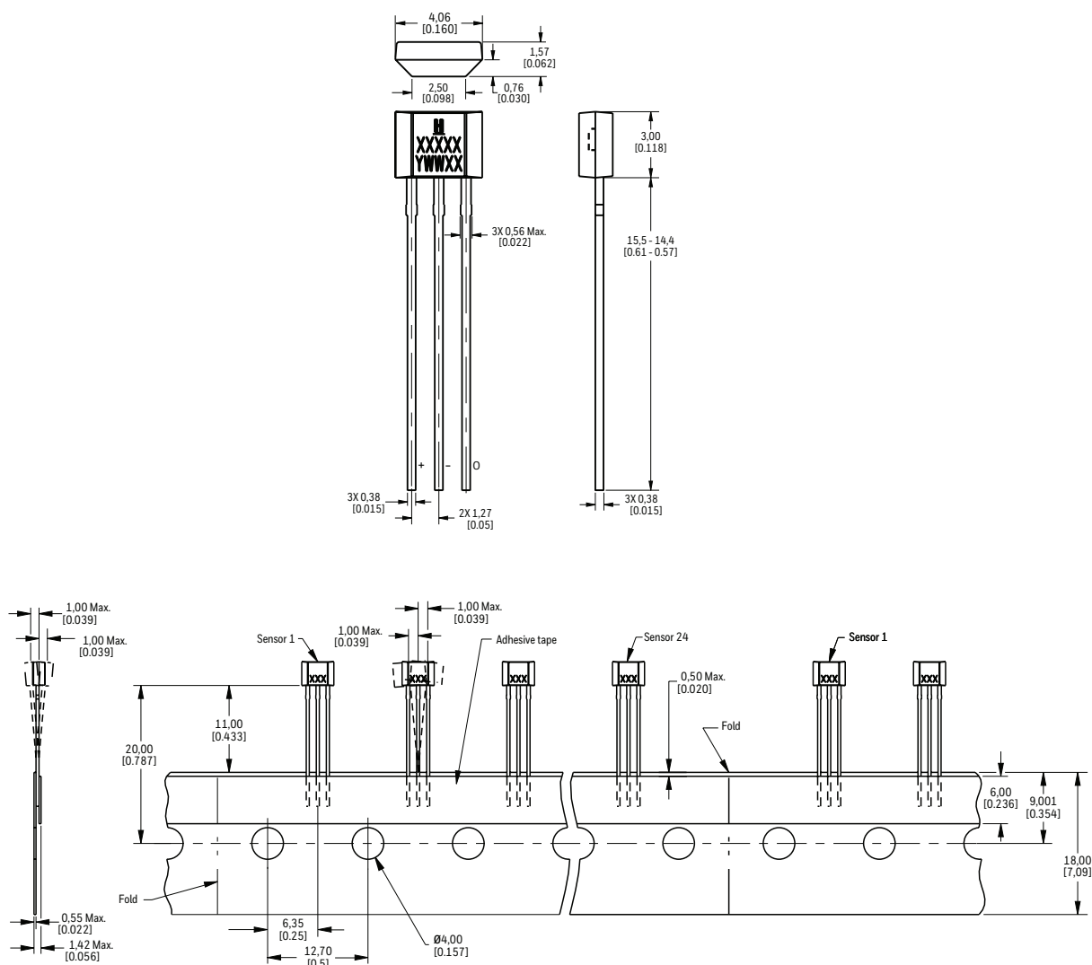
Figure 5. SS400 Series Flat TO-92-Style Mounting and Dimensional Drawings (For reference only: mm/[in].)
